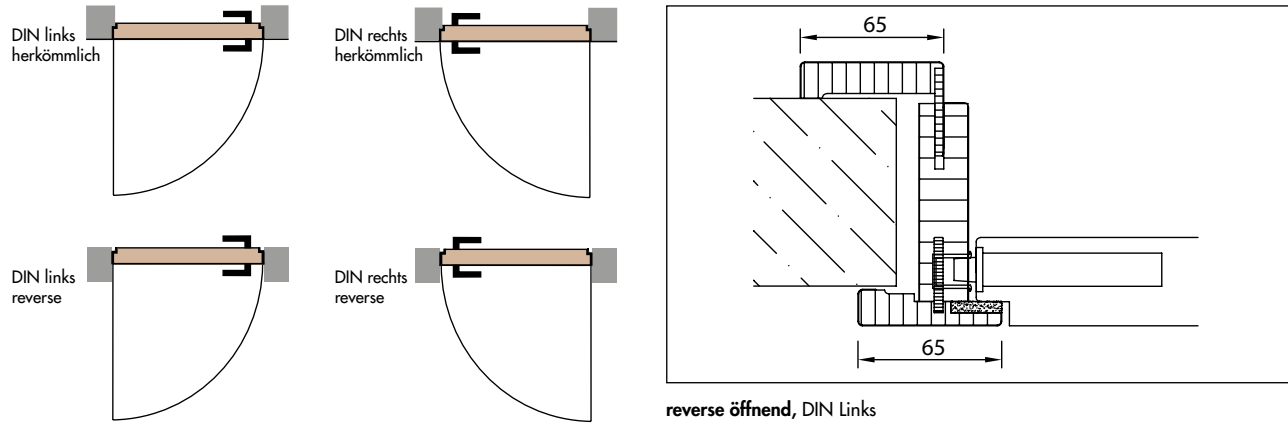
reverse öffnend, DIN Links
